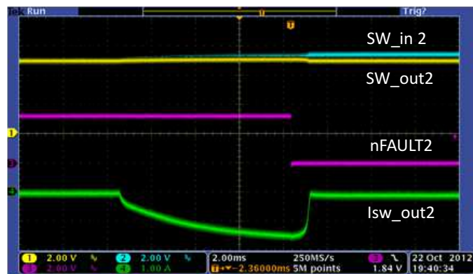
Figure 46. USB Switch2 Output Reverse Protection
